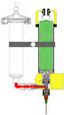
TS5000DMP-DCX Diaphragm Valve
