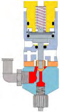
TS5620 Diaphragm Valve
