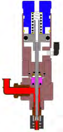
TS5420 Needle Valve
